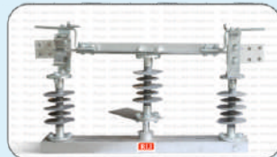
22KV - 400A Double Break Center Rotating Type
