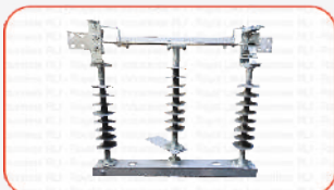
33KV 400A Double Break Centre Rotating Copper Flat Type
