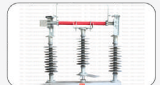
33KV Double Break Centre Rotating Type Current Rating : 400A-2000A
